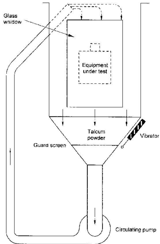
FIG. 2 APPARATUS FOR PROVIDING PROTECTION AGAINST DUST
