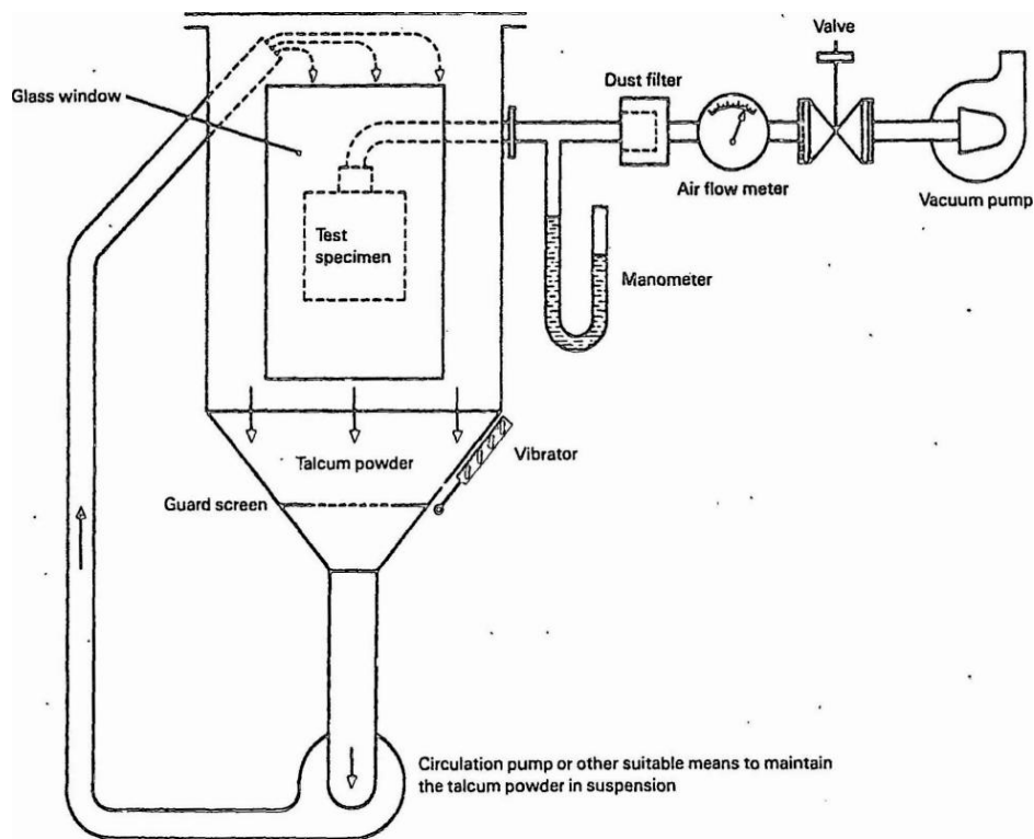
Figure 1 — Test device to verify protection against dust (dust chamber)
